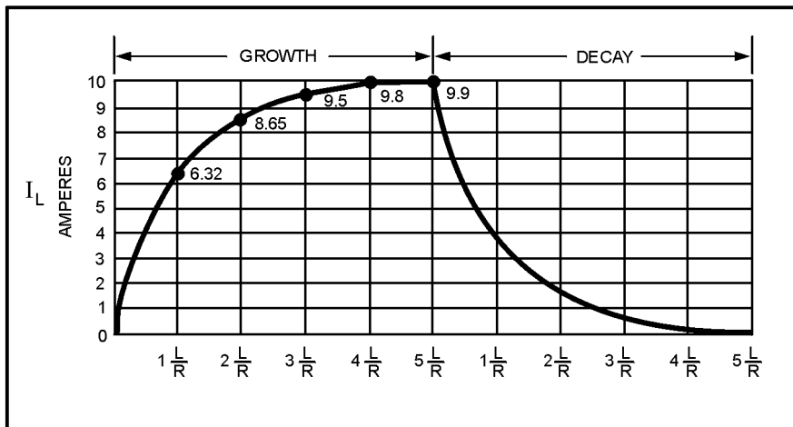
Figure 1-13.—L/R time constant.
